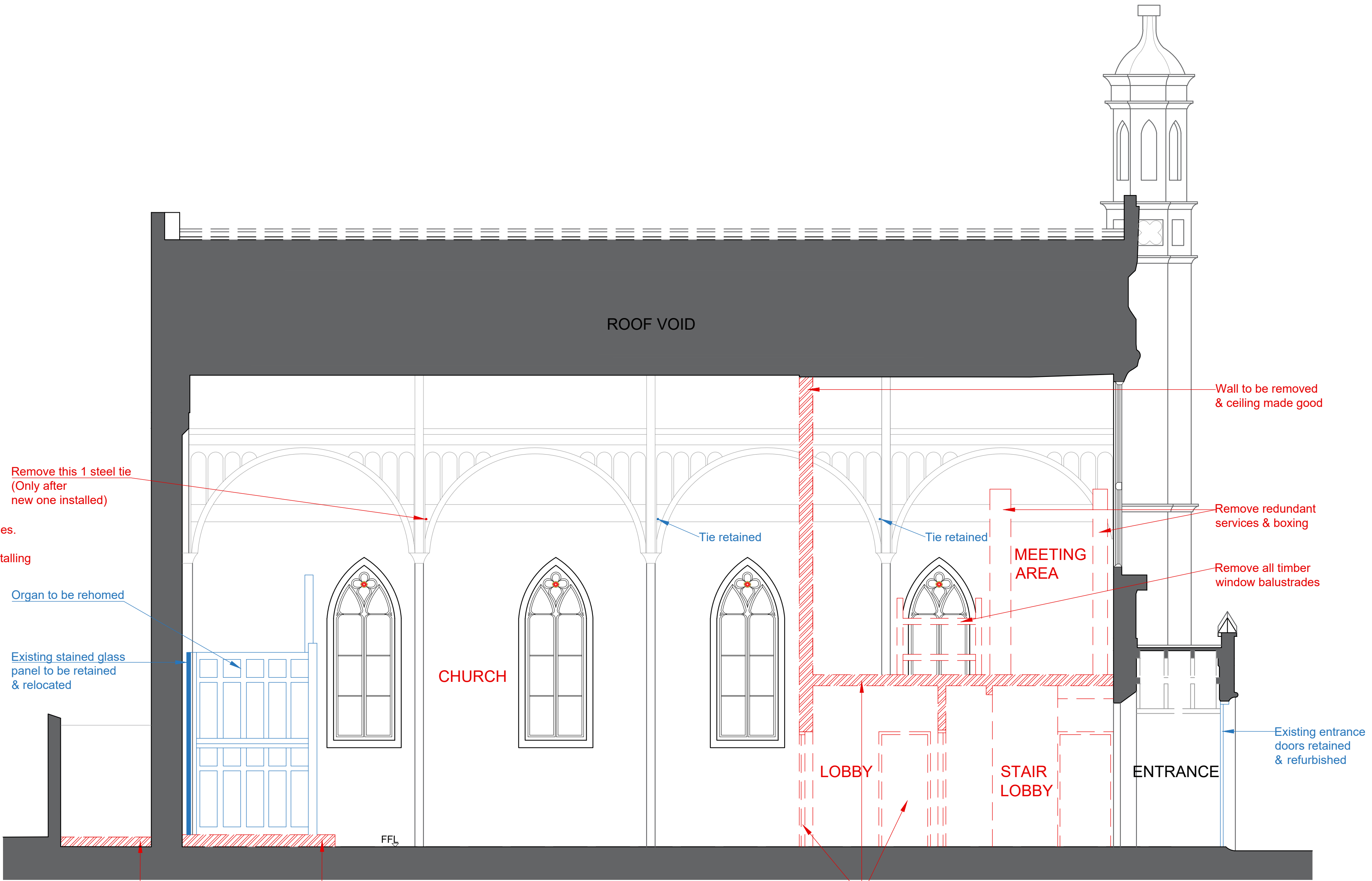
SECTION B
