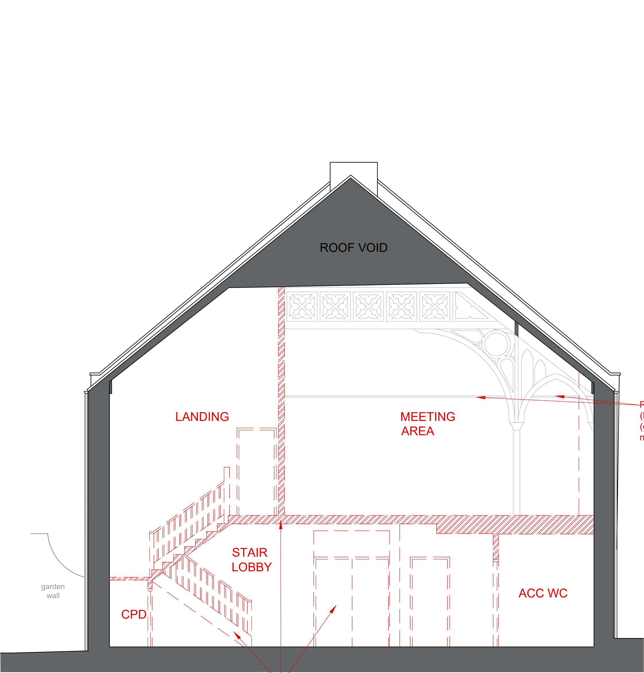
SECTION A
