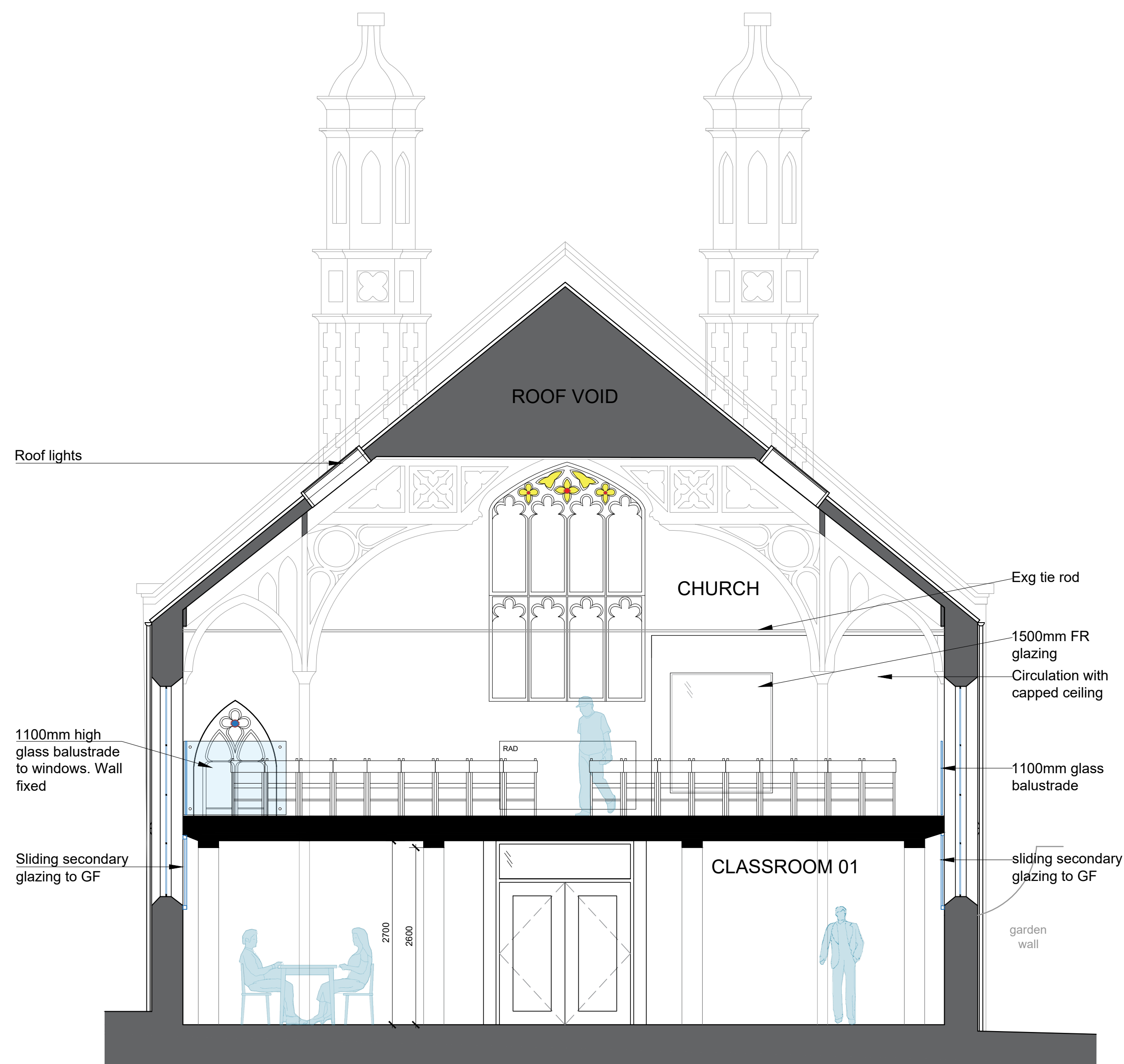
SECTION C-C
