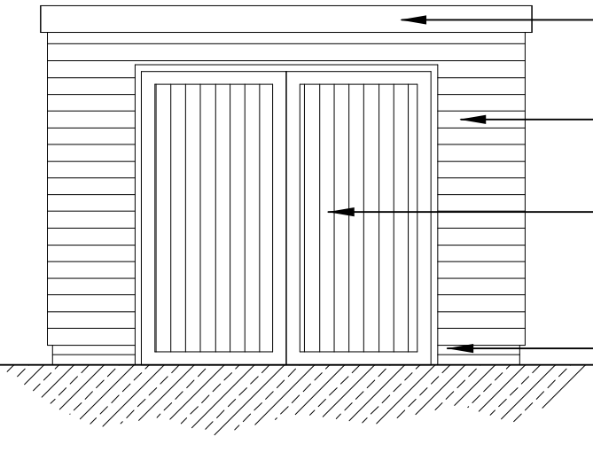
PROPOSED ELEVATION F (FRONT)
