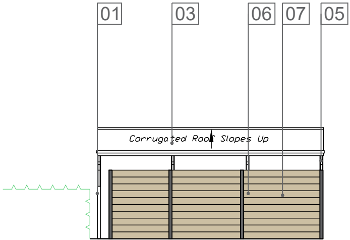
Elevation 2 1:100@A3
