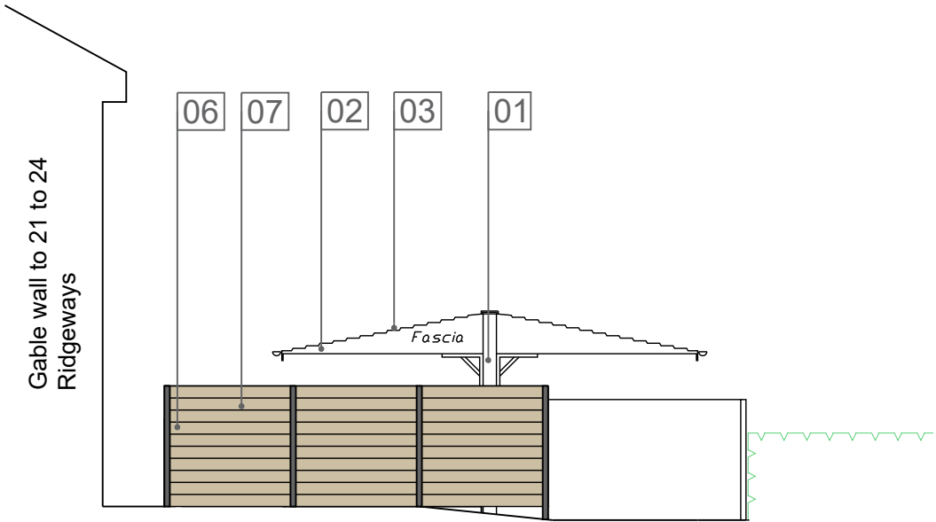
Elevation 1 1:100@A3
