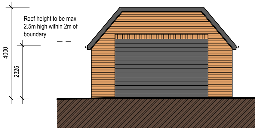
Proposed East Elevation 1 : 100
