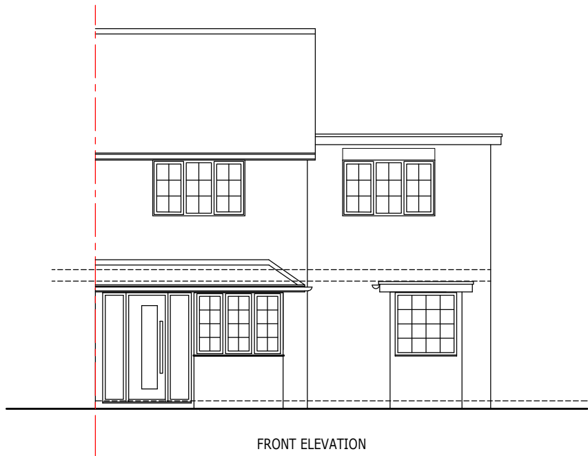
Front Elevation @ 1/100
