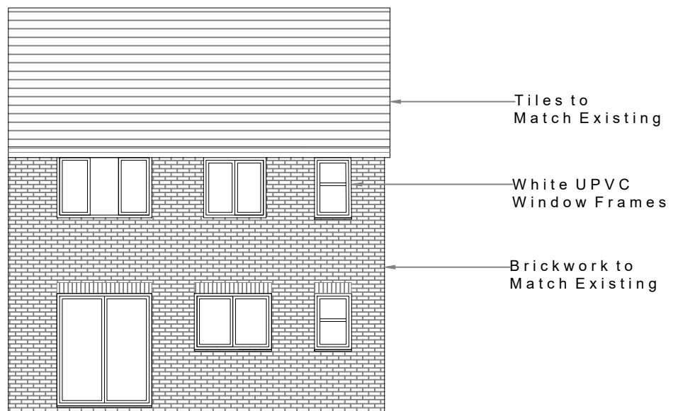
Rear Elevation
