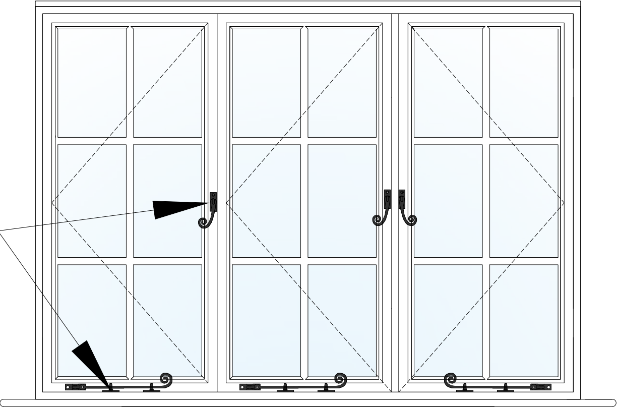
WINDOW A - Proposed Internal View (1:10)
