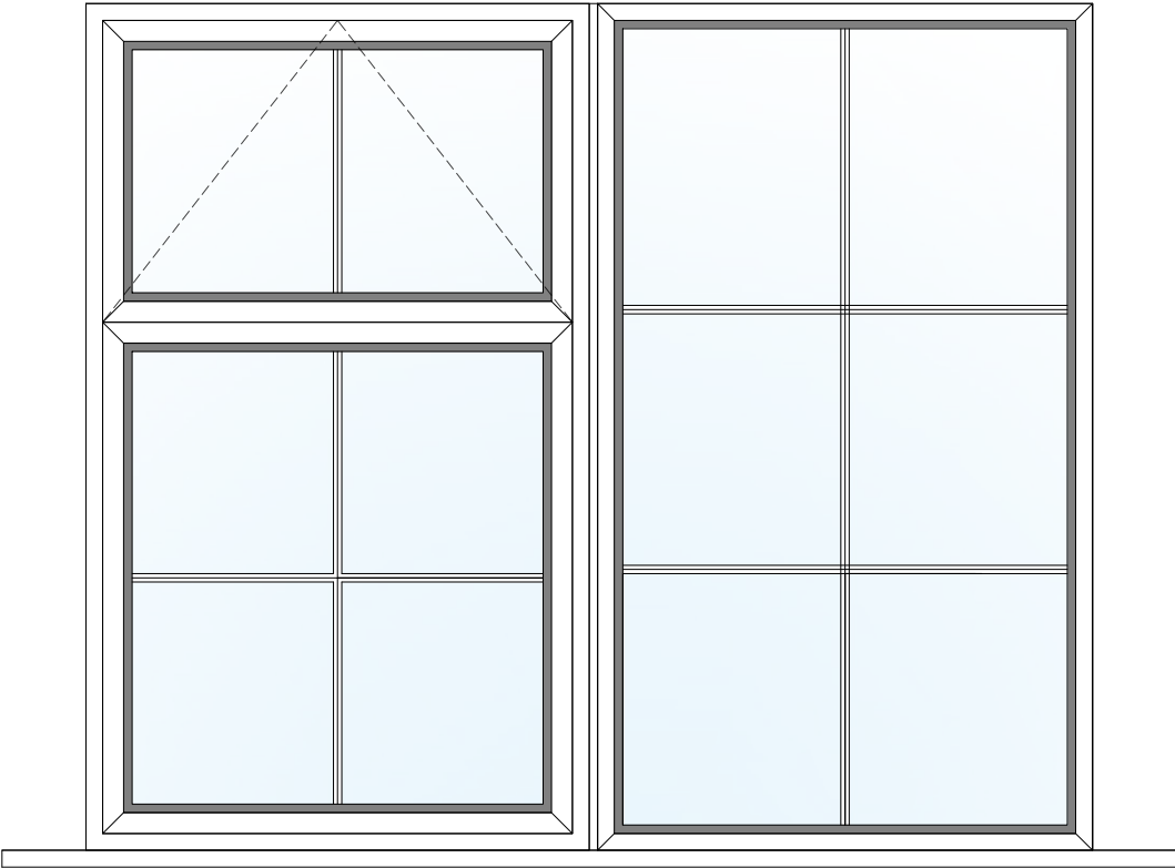
WINDOW B - Existing External View (1:10)
