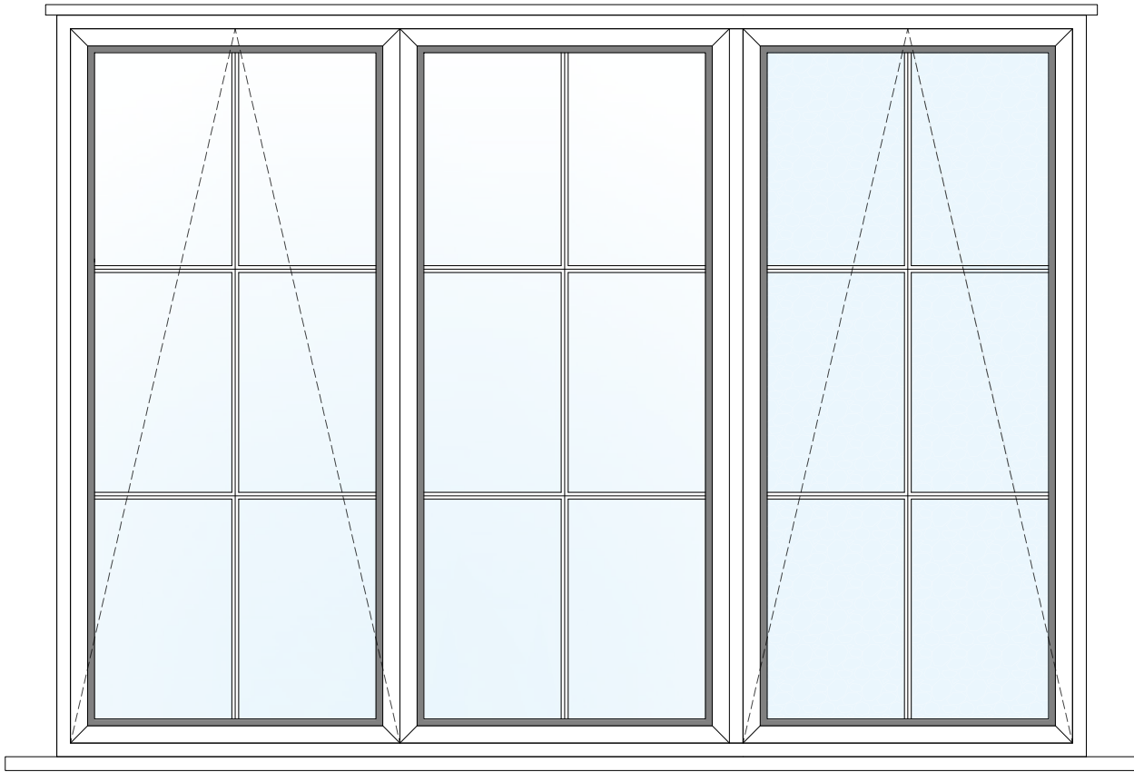
WINDOW A - Existing External View (1:10)
