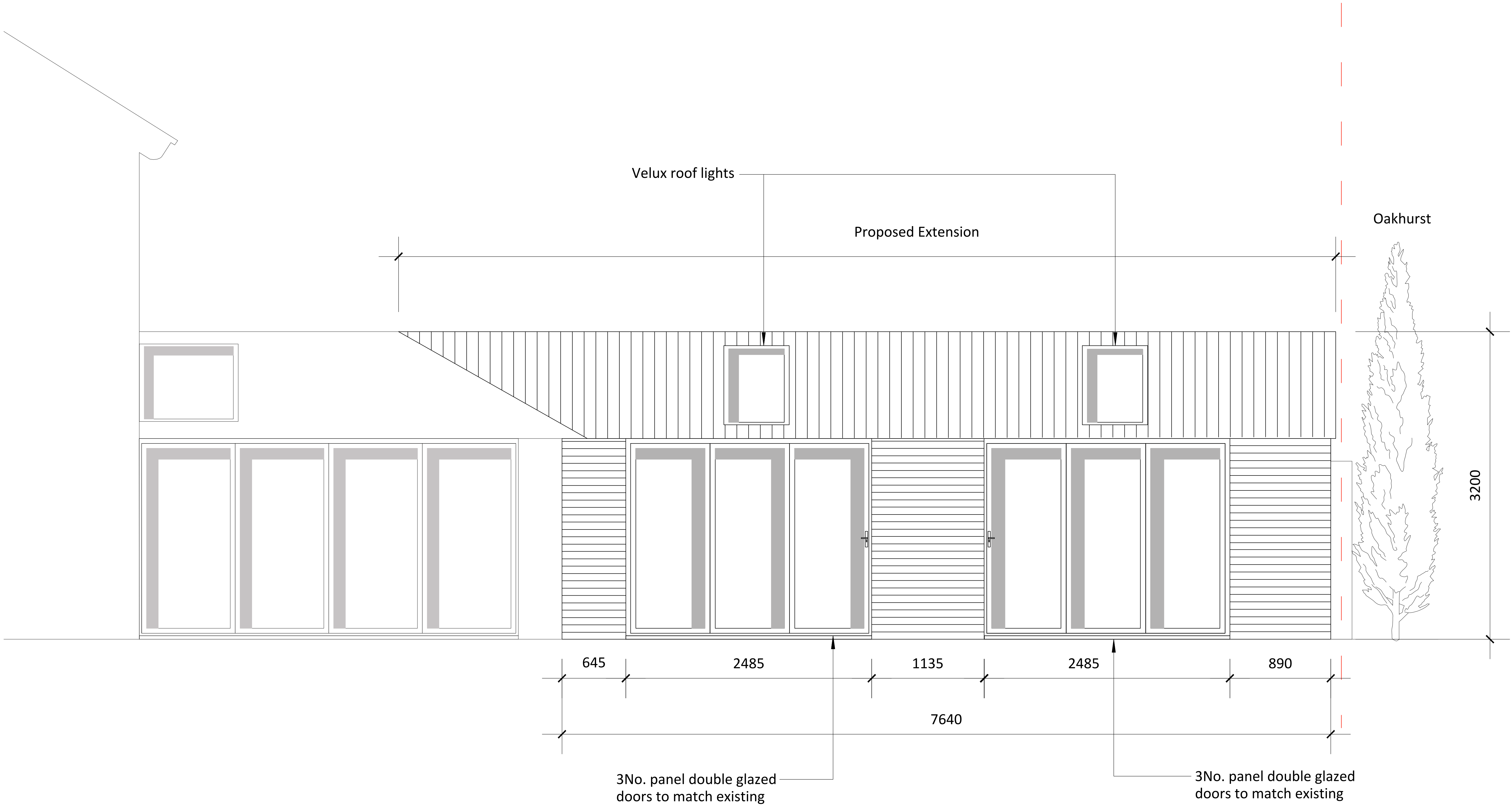
Proposed Extension North West Elevation
