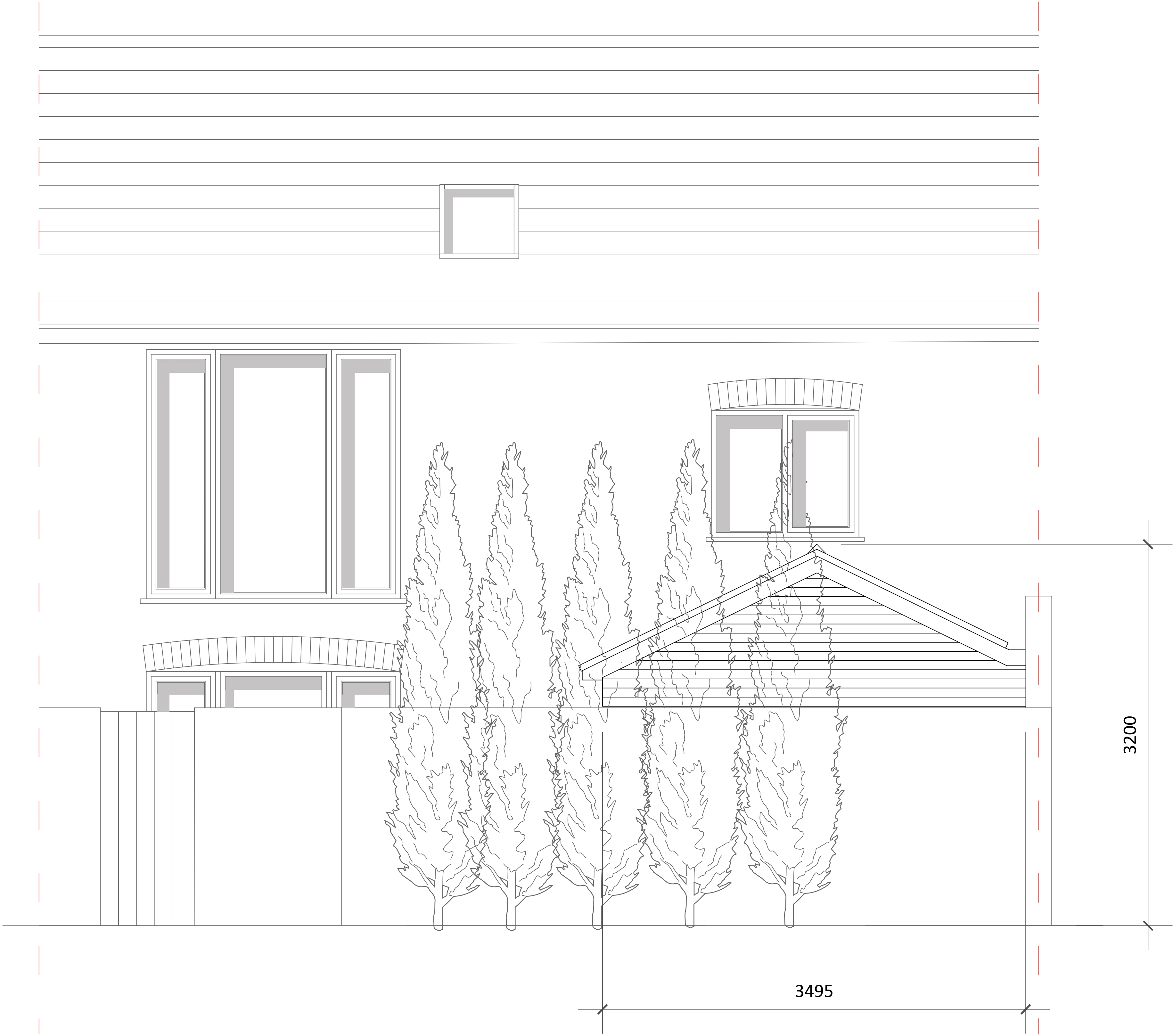
Proposed Extension South West Elevation
