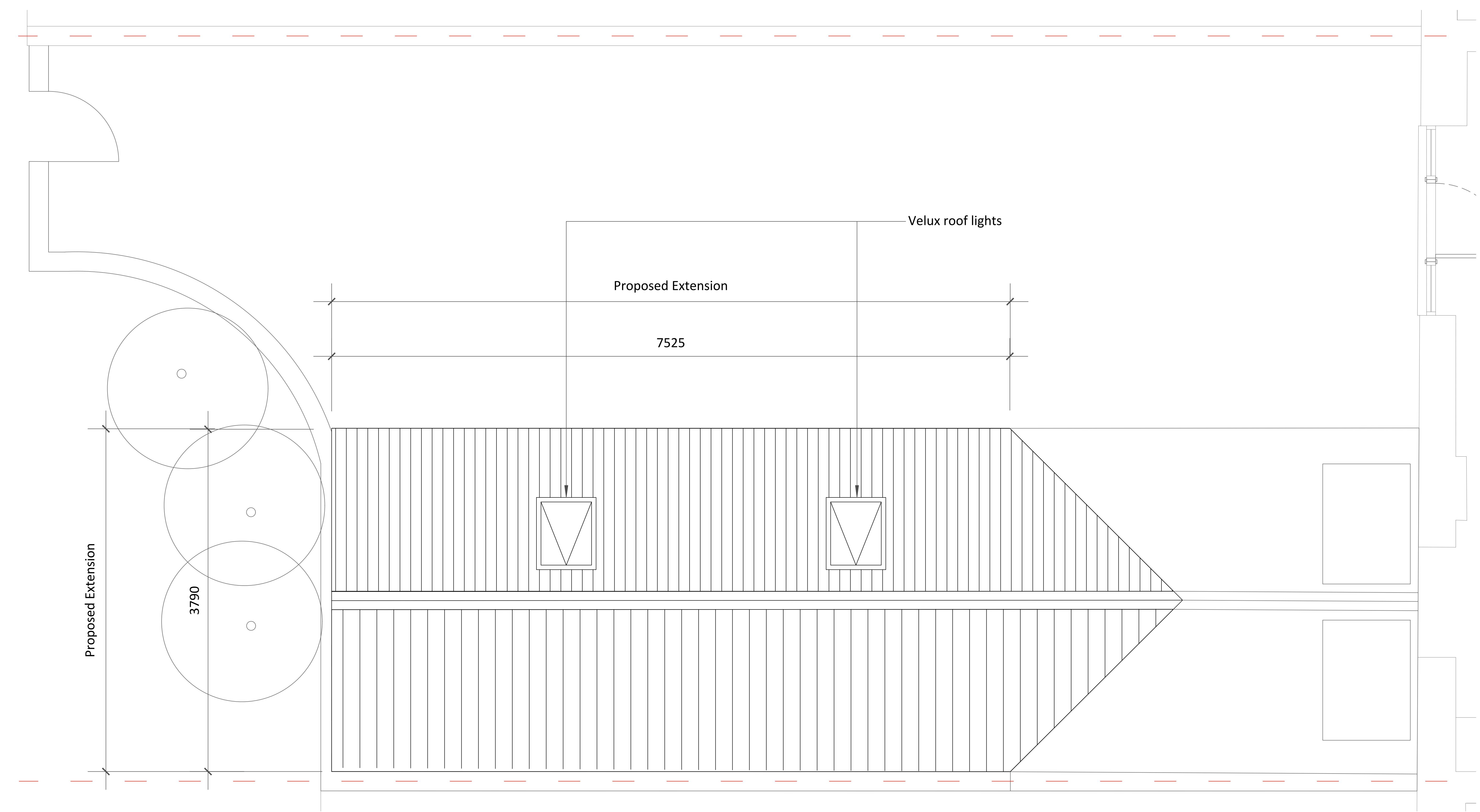
Proposed Extension Roof Plan
