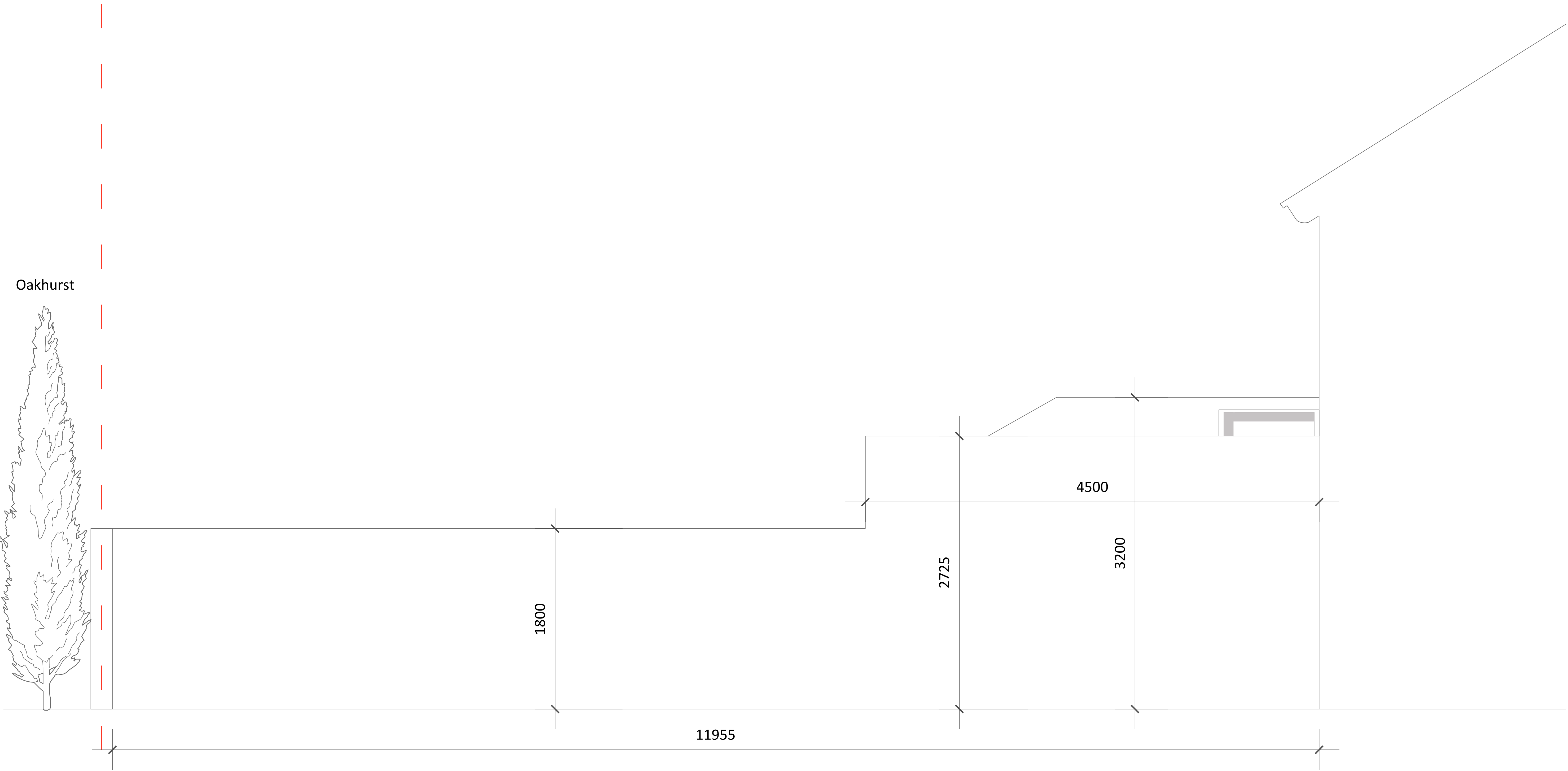
Existing South East Elevation
