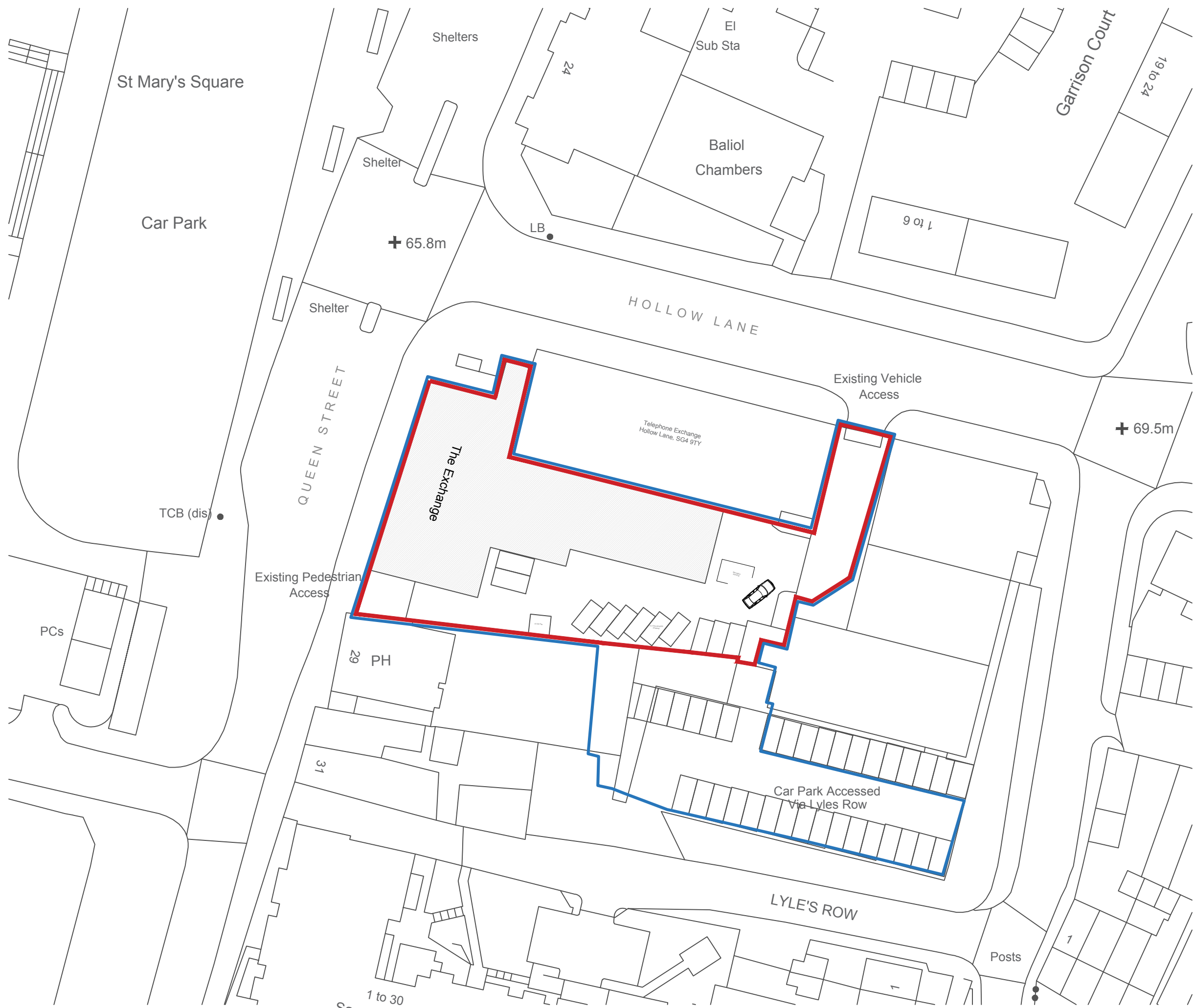
EXISTING SITE LAYOUT PLAN
