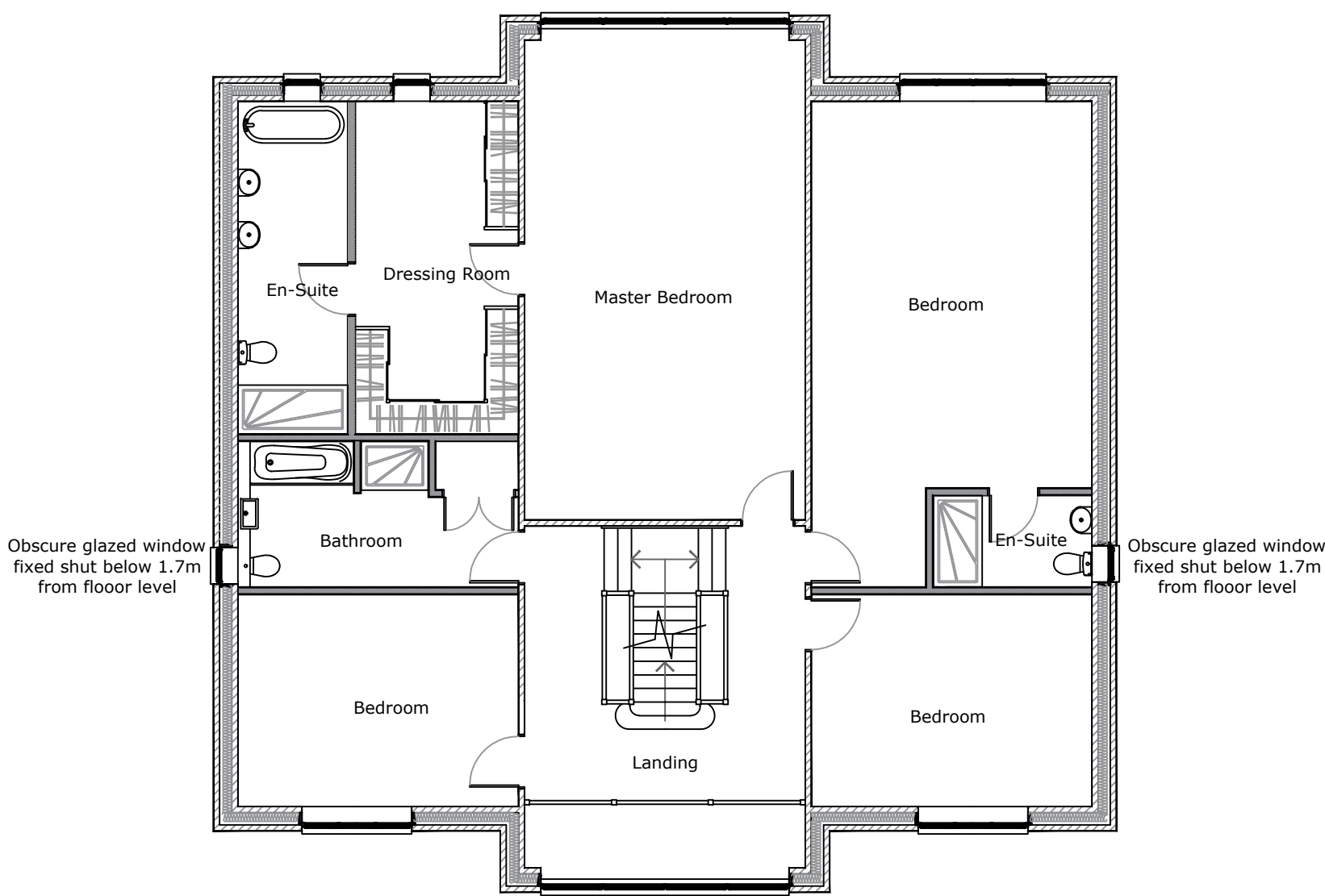
House 1st Floor Plan 1:100
