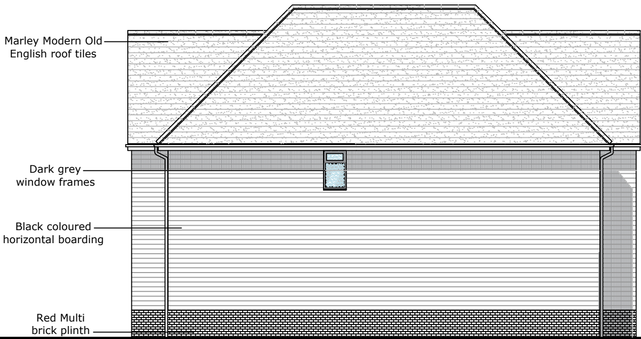
House Elevation Side 1:100
