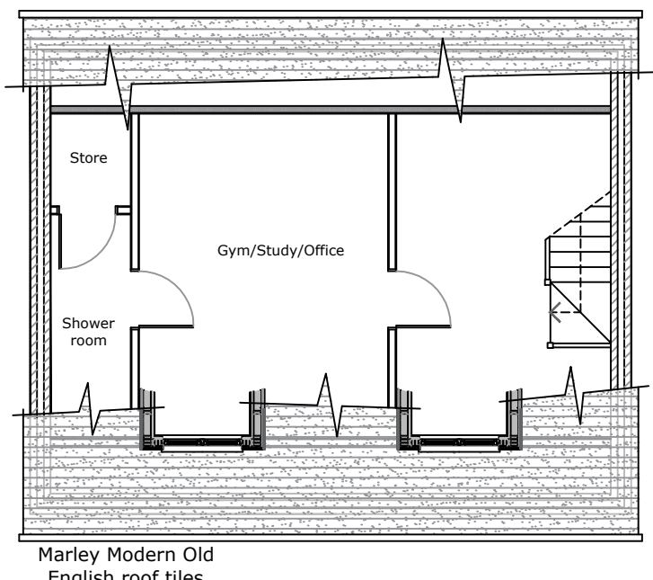
Garage 1st Floor Plan 1:100
