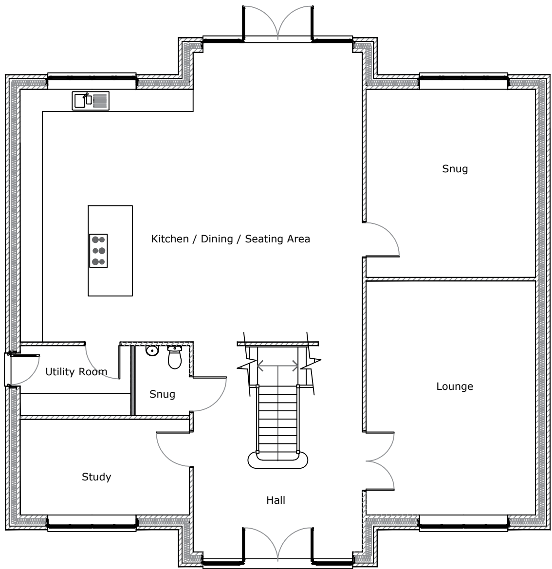
House Ground Floor Plan 1:100
