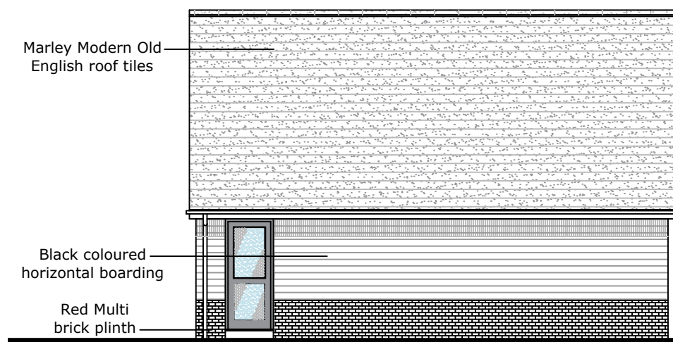
Garage Elevation Rear 1:100
