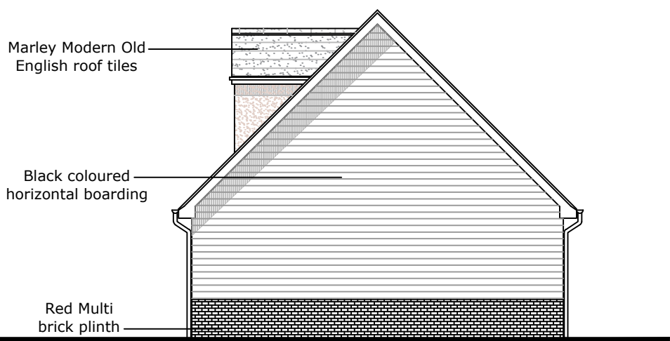
Garage Elevation Side 1:100
