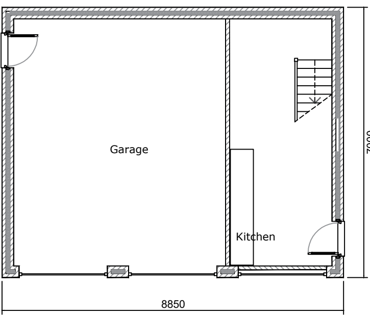
Garage Ground Floor Plan 1:100
