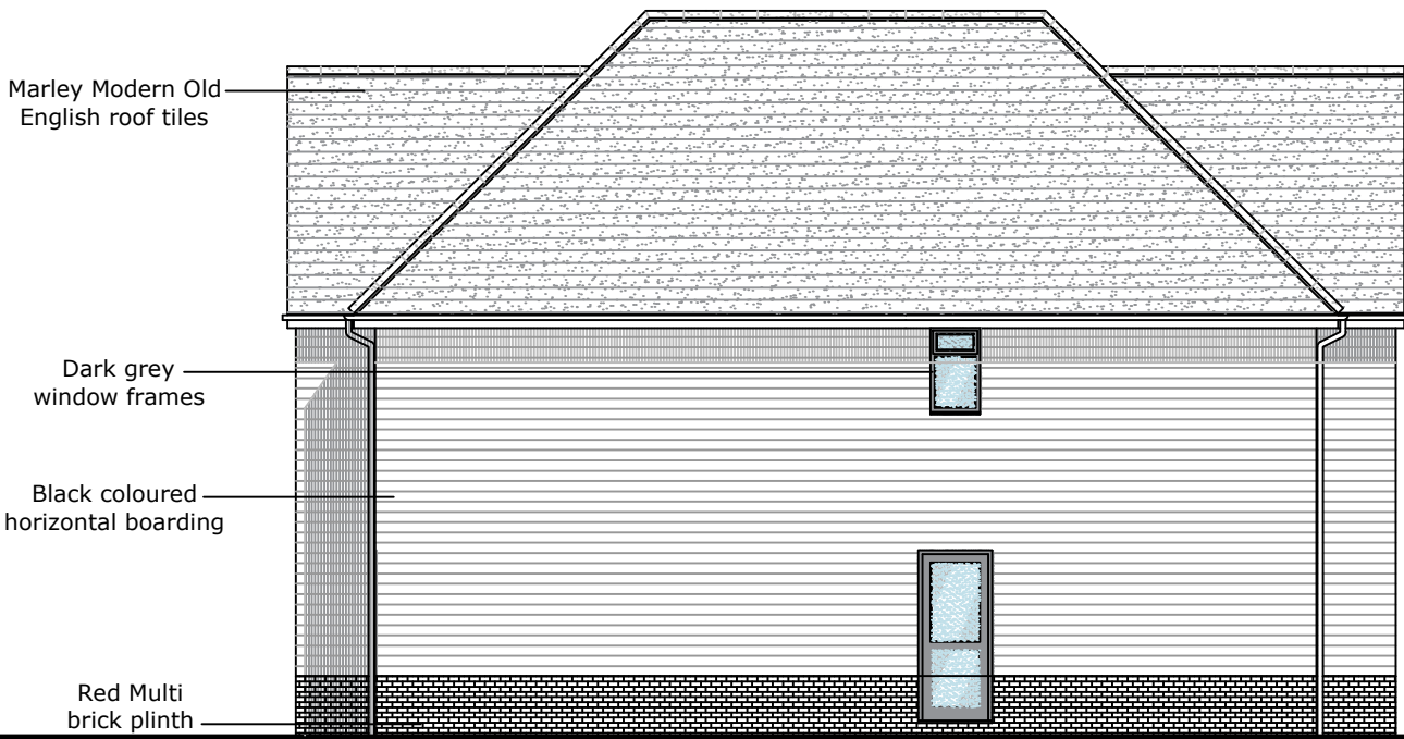
House Elevation Side 1:100
