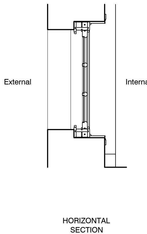
STAIRWELL WINDOW SECTIONS (W2) (1:20)
