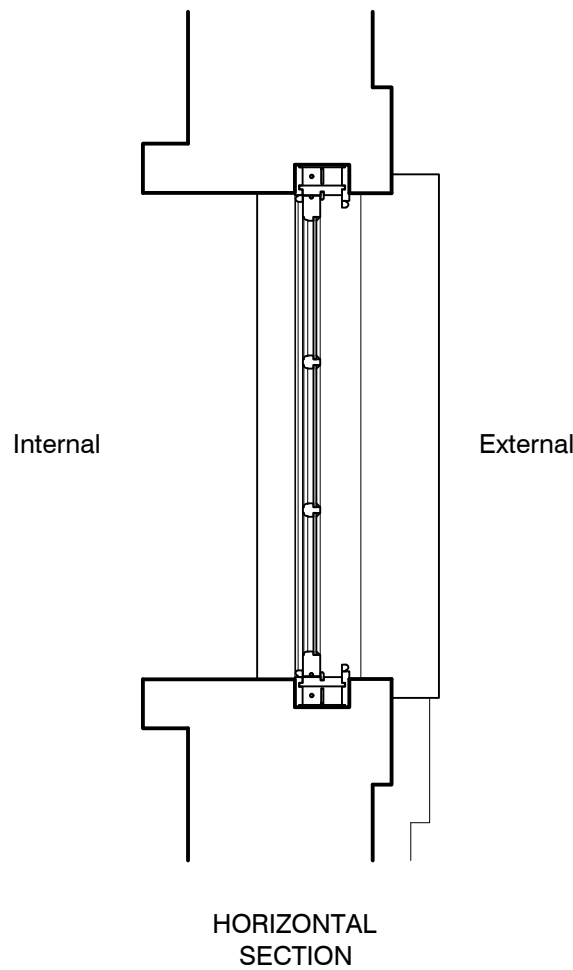
MAIN WINDOW SECTIONS (W1) (1:20)
