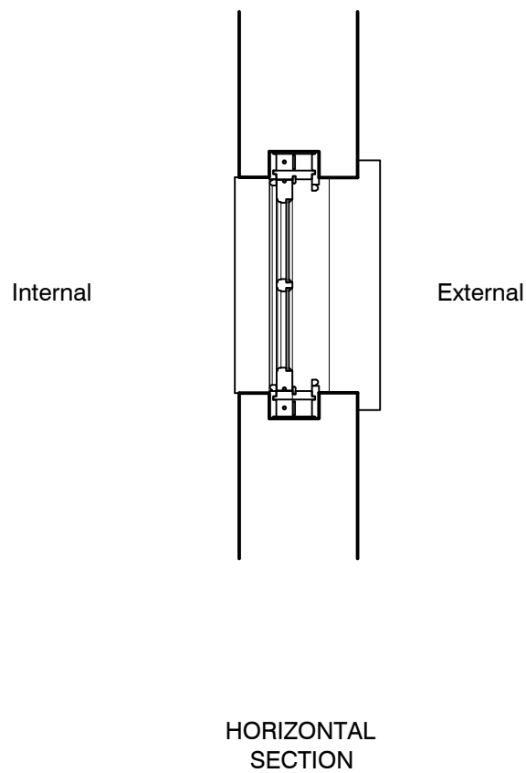
ANNEXE WINDOW SECTIONS (W3) (1:20)
