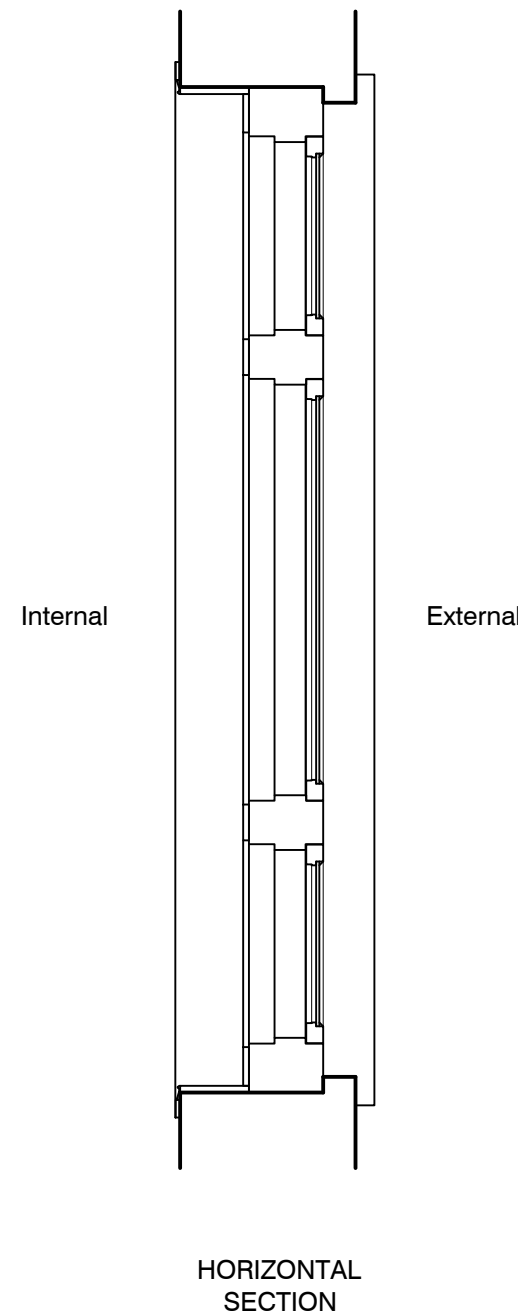
LOUNGE/DINING ROOM WINDOW SECTIONS (W4) (1:20)
