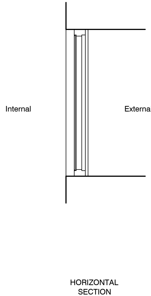
BASEMENT WINDOW SECTIONS (W5) (1:20)
