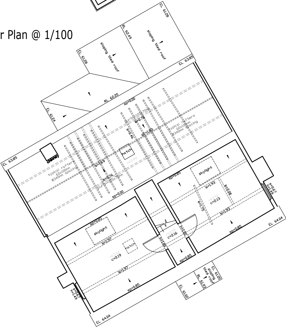
Roof Plan @ 1/100
