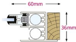
Jamb detail lower sash
