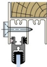
Screw lock
