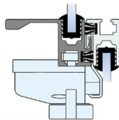
Fitch catch
