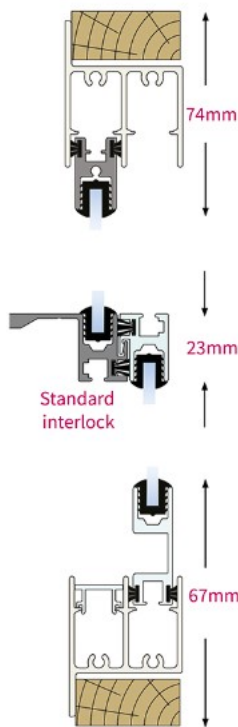
Jamb detail lower sash
