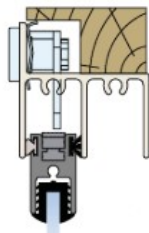
Key lock
